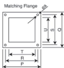
Matching Flange
