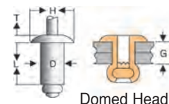
Domed Head
