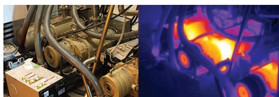
Failing Pumps/Motors
