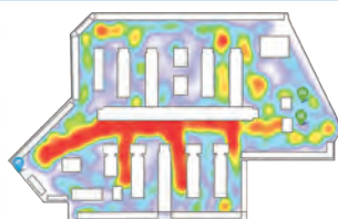
Density Heatmaps
